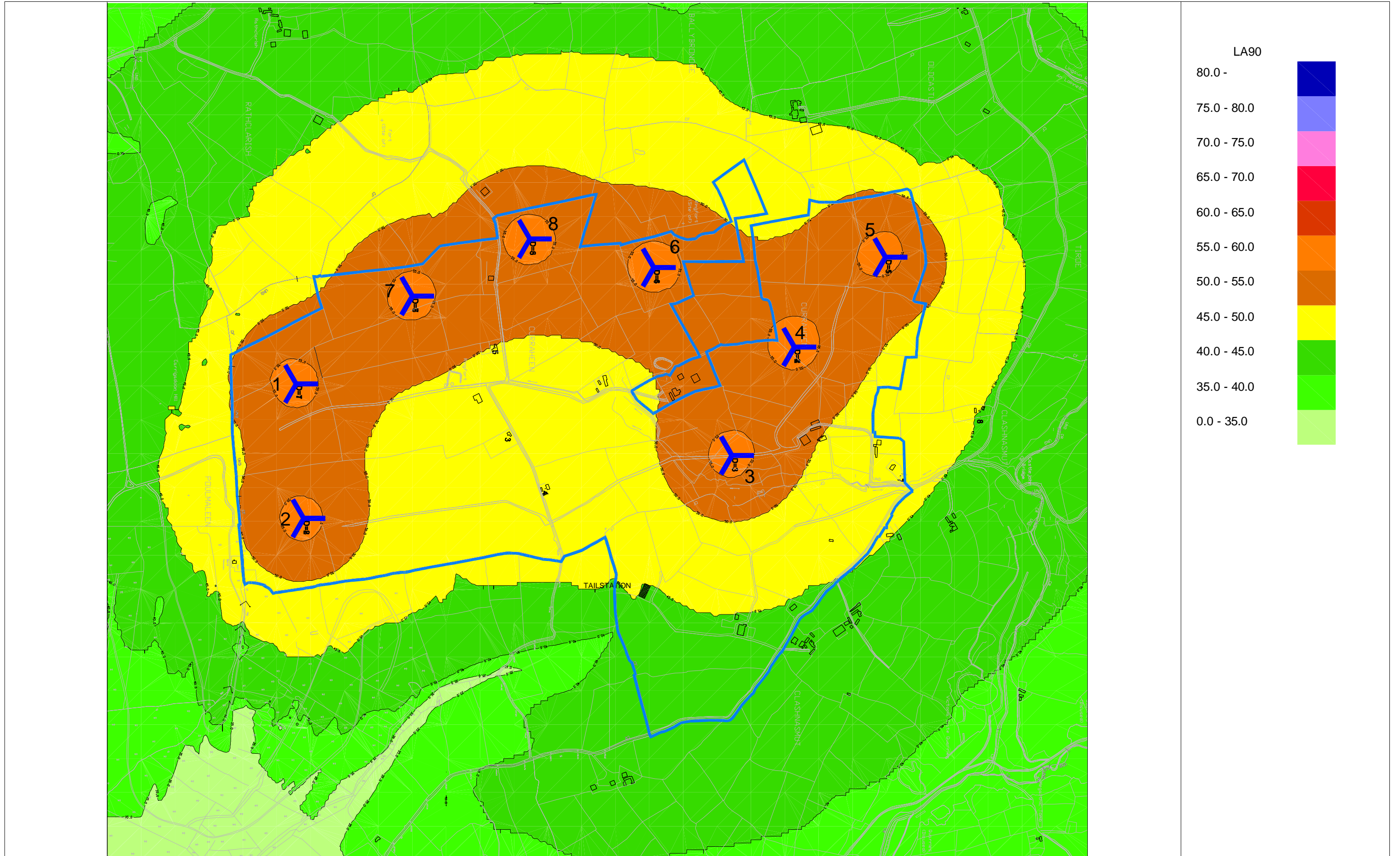
NOISE MAP WITH 8m CONTOURS FIGURE 10.3
